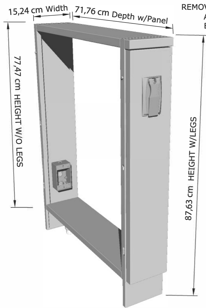
ISO VIEW
