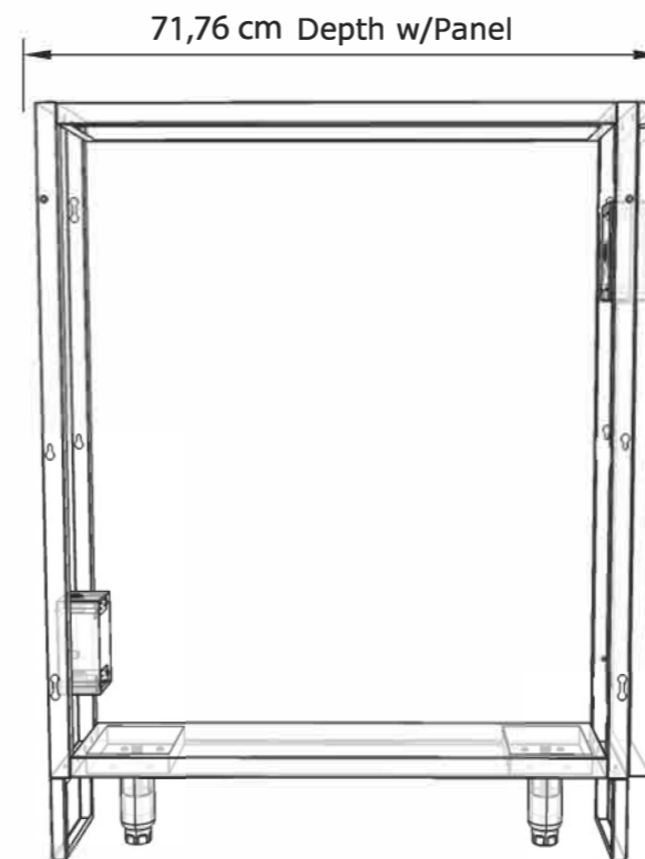
TOP VIEW
